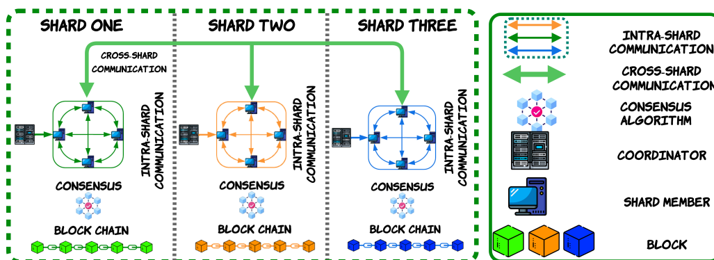
Figure 9. The diagram illustrates category-based sharding, dividing a blockchain into categories with dedicated shards for data storage. A coordinator manages shards, and a lookup table directs category queries. Intra-shard and cross-shard communication occurs via a peer-to-peer network.
