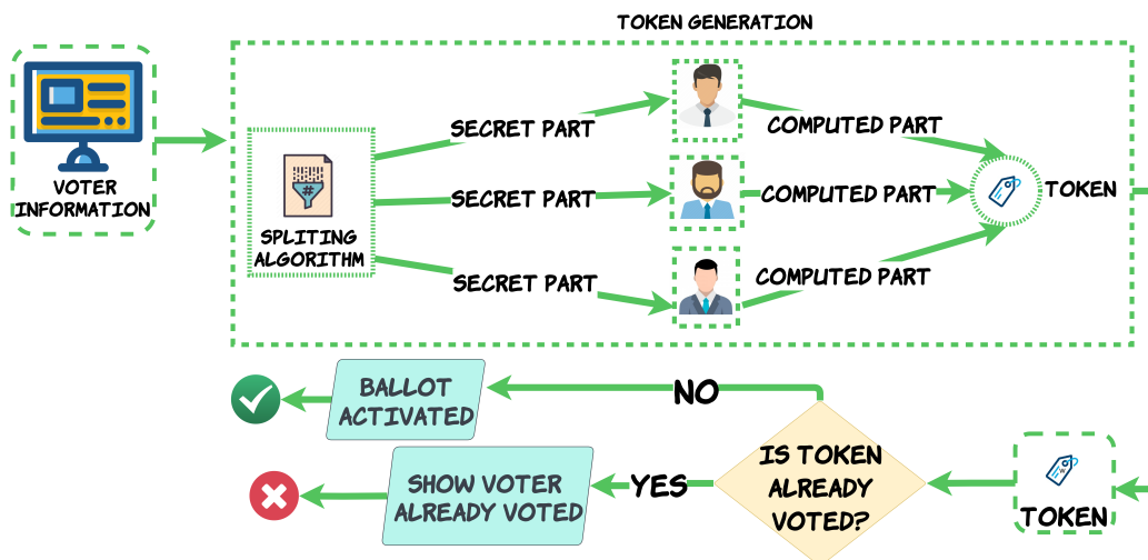
Figure 11. The high-level representation of the structure of token-based verification in the system shows how voter information is split and computed into a token, which is then used to verify double voting without revealing the voter’s identity.
